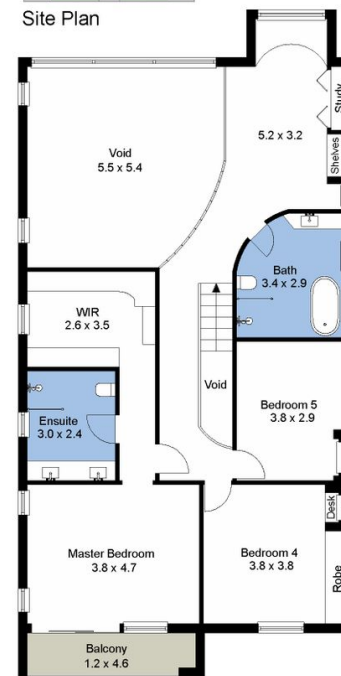
1st Floor
